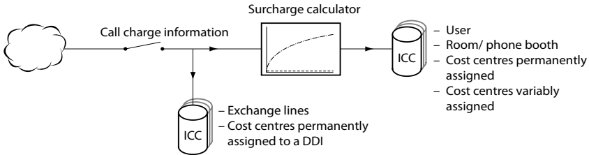
Fig. 128 Call charge allocation
