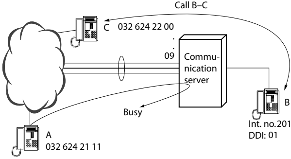
Fig. 158 Call to a busy user
