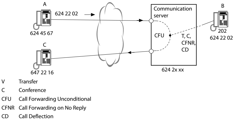
Fig. 102 Exchange-to-Exchange Connection
