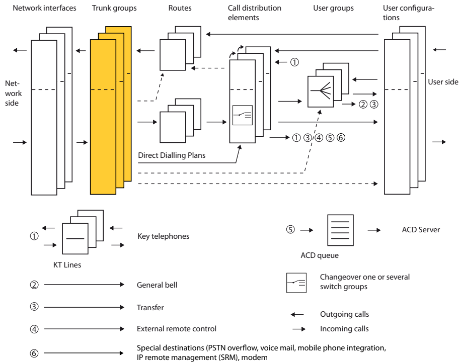
Fig. 45 Trunk groups in relation to the other routing elements
