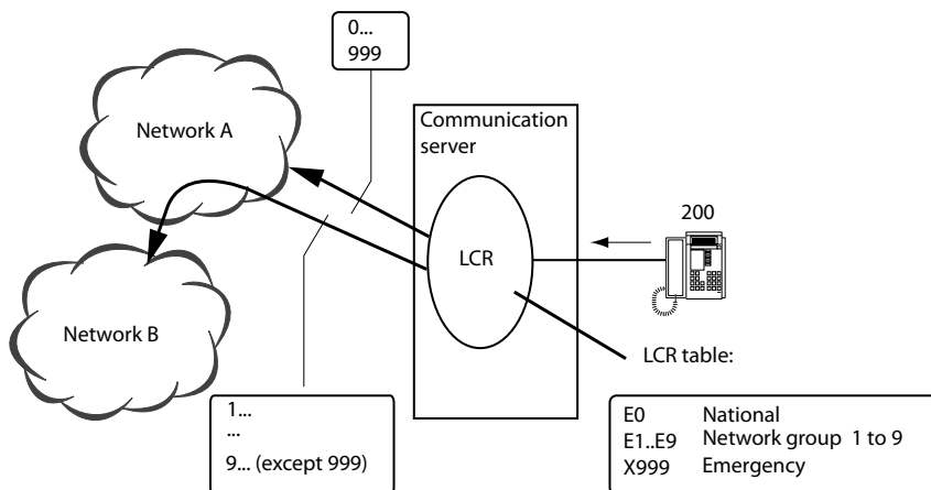
Fig. 98 Routing the emergency number 999
