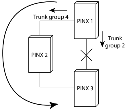
Fig. 116 Overflow routing in the private leased-line network using a sensible trunk group allocation in the route configuration
