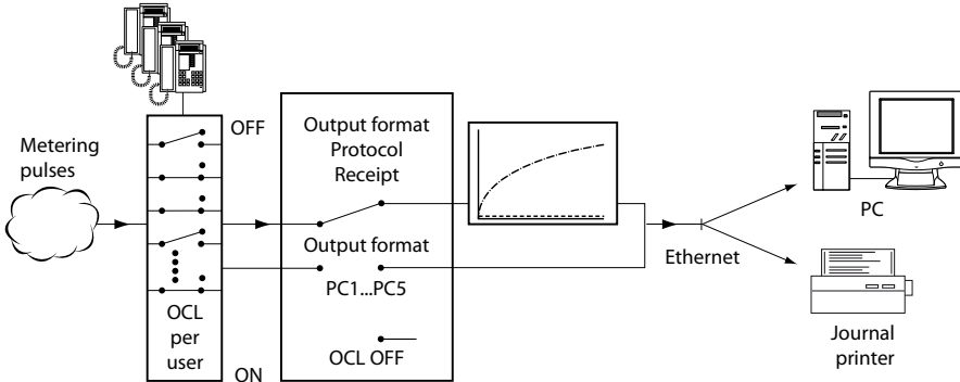
Fig. 140 Schematic sequence
