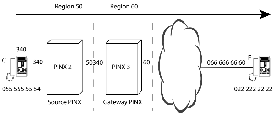
Fig. 39 Example 4: User C calls user F via an alternative path (excerpt from Fig. 35)
