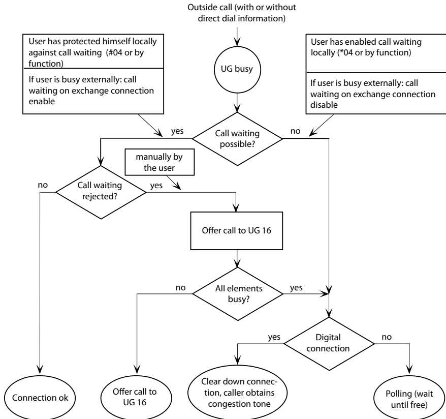
Fig. 83 Call distribution if user group busy
