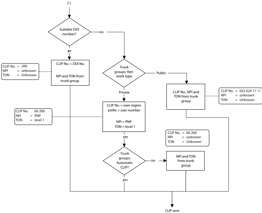
Fig. 32 Creating an automatic CLIP for outgoing calls
