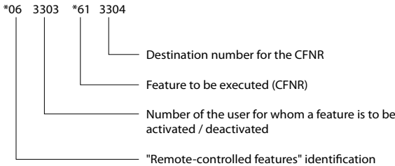
Fig. 235 Example of remote control
