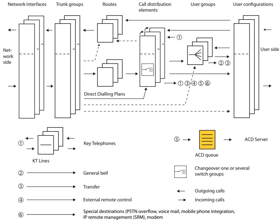
Fig. 72 The ACD server in relation to the other routing elements
