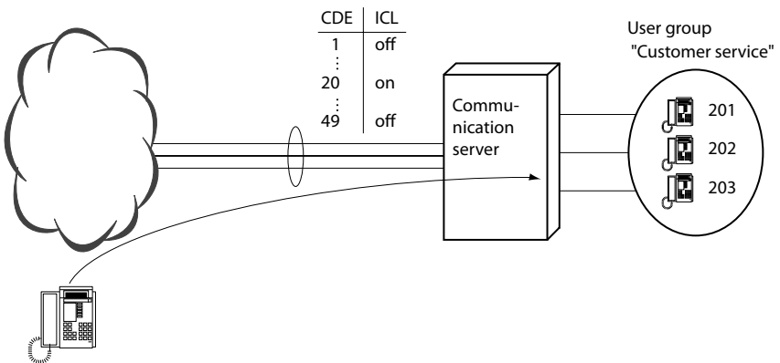
Fig. 147 ICL can be switched on or off in each call distribution element
