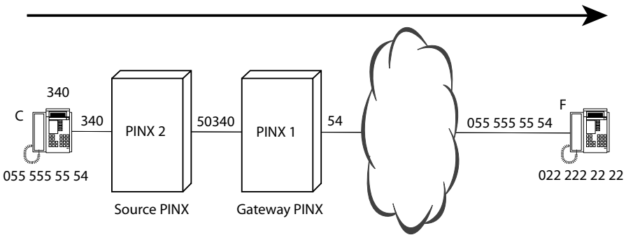
Fig. 38 Example 3: User C calls user F in the public network (excerpt from Fig. 35)
