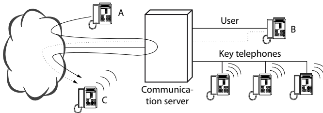
Fig. 181 DDI number to user + KT and user + KT busy
