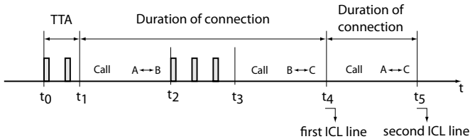
Fig. 161 Time phases for a transferred call with prior notice
