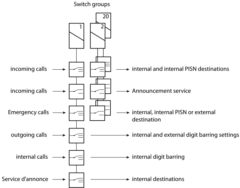
Fig. 57 Switch groups and how their changeover switches are used
