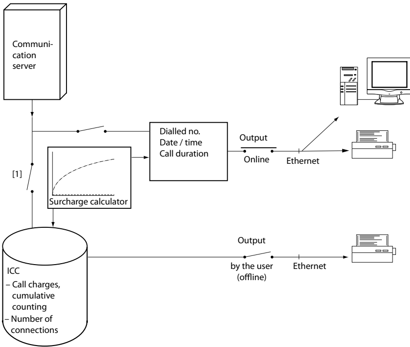
Fig. 126 Call logging and charge acquisition for outgoing traffic
