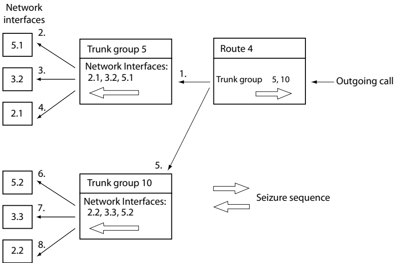
Fig. 48 Seizure sequence for network connections in the case of an outgoing call
