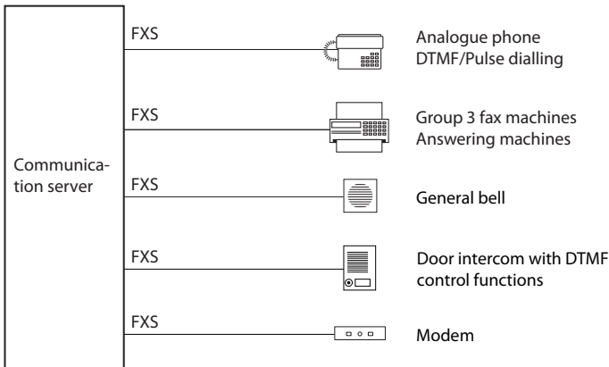
Fig. 16 FXS terminal interface
