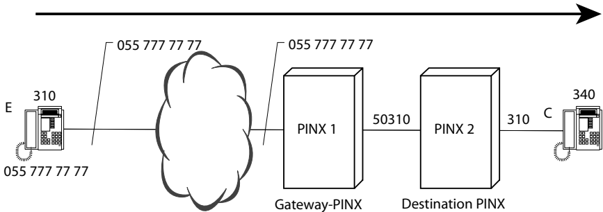
Fig. 43 Example 8: User E calls user C (excerpt from Fig. 35)
