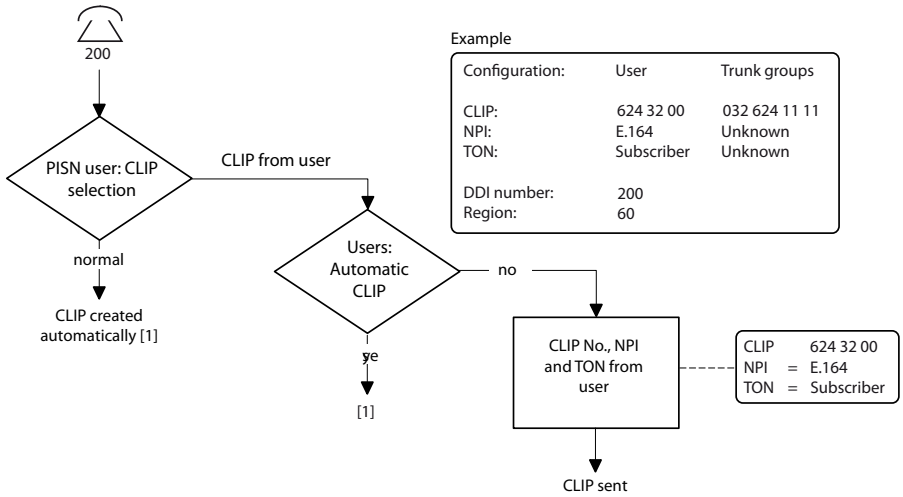
Fig. 31 CLIP of an outgoing call to a PISN user
