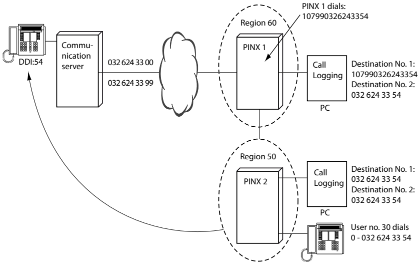
Fig. 152 Destination number outgoing
