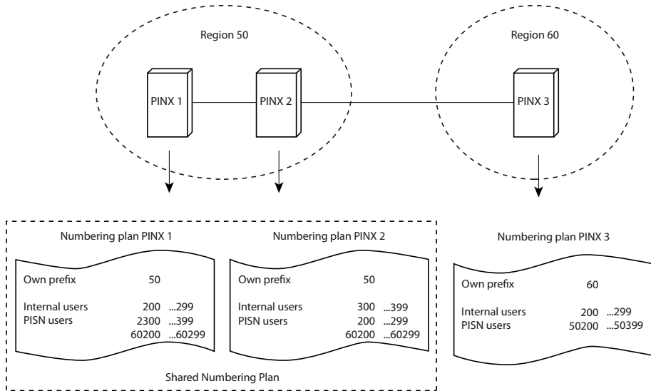
Fig. 22 PISN with two regions and shared numbering plan for Region 50
