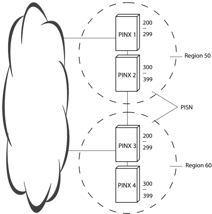
Fig. 20 PISN with two regions
