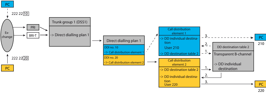
Fig. 122 Incoming data-service routing from the public network with direct dialling to a data-service individual destination
