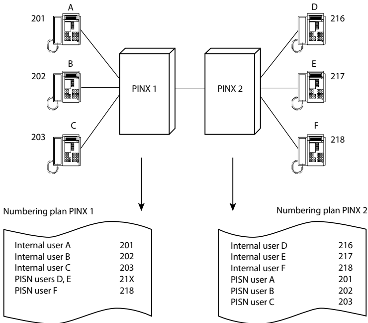
Fig. 19 PISN users entered with and without wildcards
