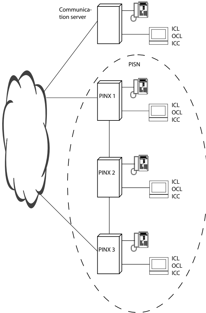
Fig. 127 Call logging in the PISN
