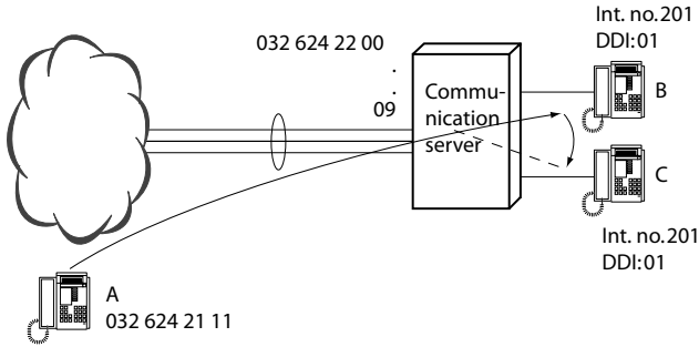
Fig. 159 Transferred call
