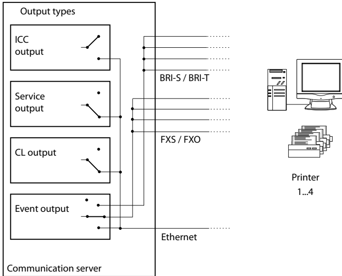
Fig. 148 Output concept
