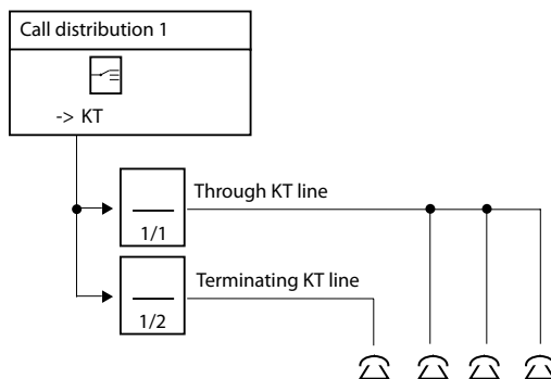
Fig. 68 Through and terminating KT lines
