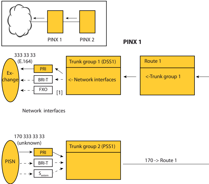
Fig. 113 Transit routing for private leased-line network → public network with exchange access prefix
