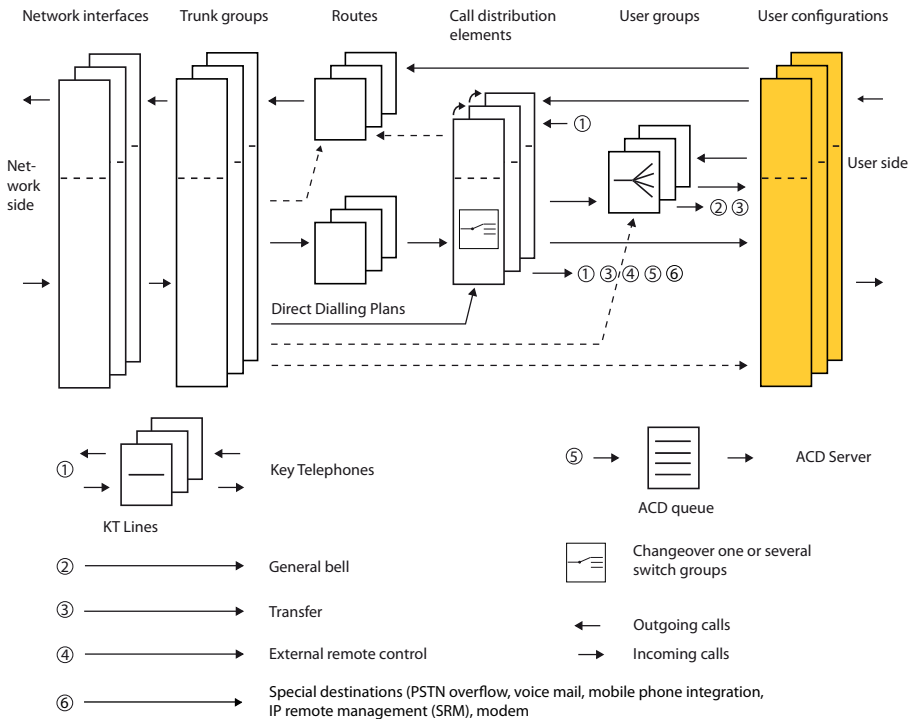
Fig. 64 User configuration in relation to the other routing elements
