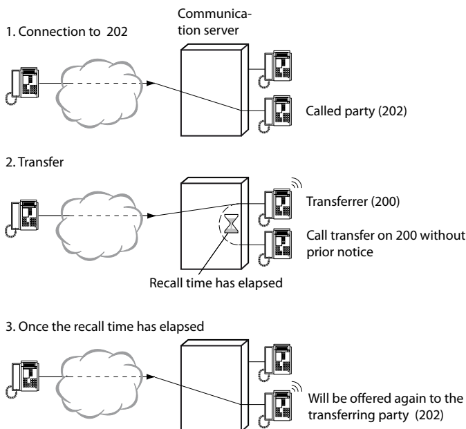
Fig. 199 Recall time
