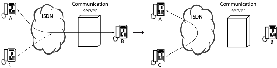
Fig. 108 Brokering followed by call transfer
