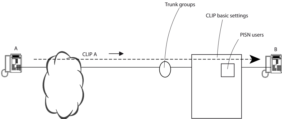
Fig. 33 CLIP incoming
