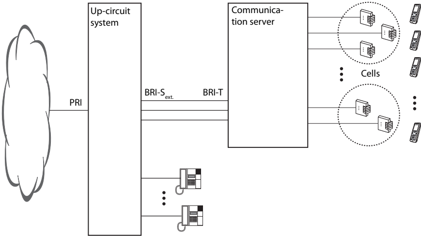
Fig. 9 Digital down-circuit connection with QSIG
