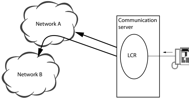
Fig. 95 Indirect access to network B via network A using LCR
