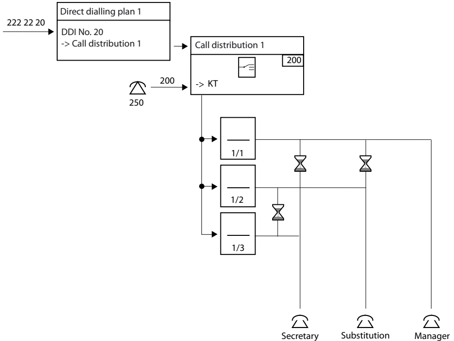
Fig. 71 Substitution circuit with key telephones
