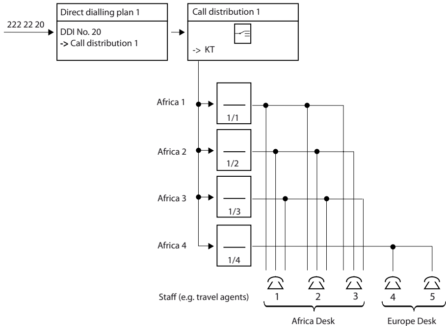
Fig. 70 Substitution Circuit
