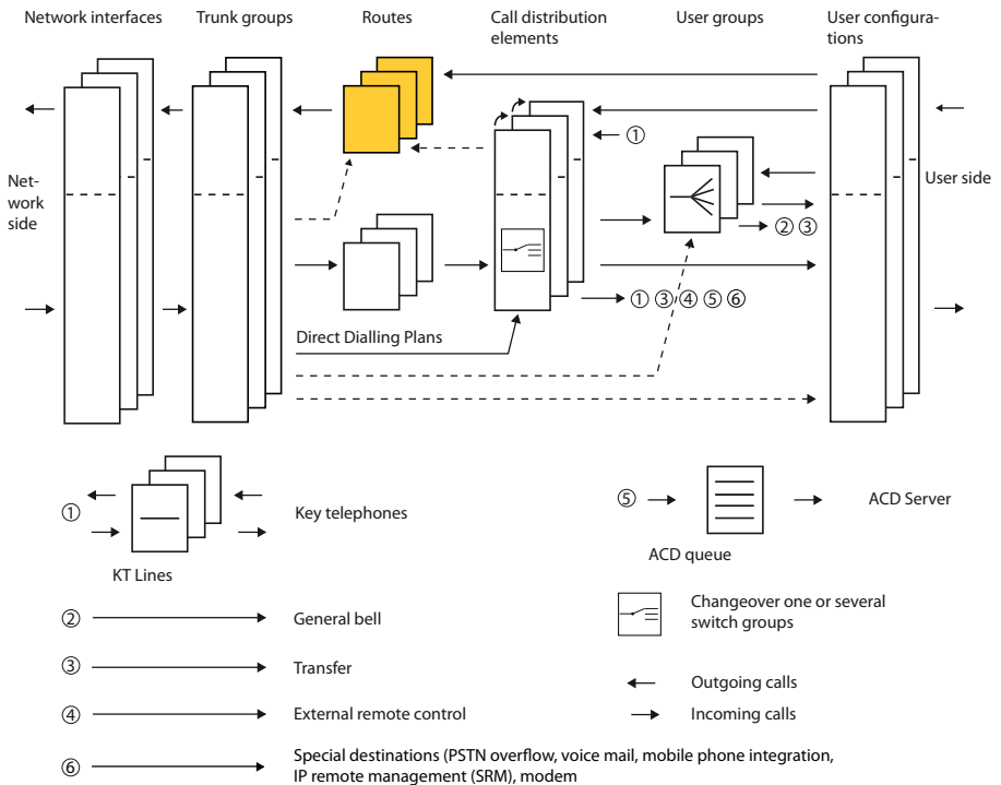
Fig. 47 Routes in relation to the other routing elements
